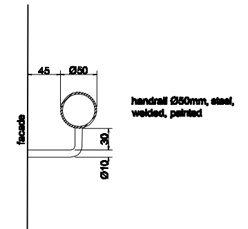
detail handrail 1:5
