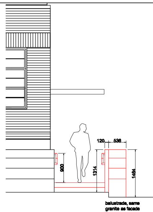
side elevation 1:50
