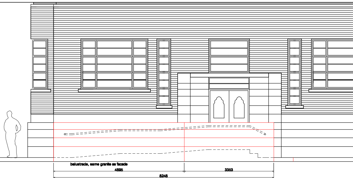
main elevation 1:50
