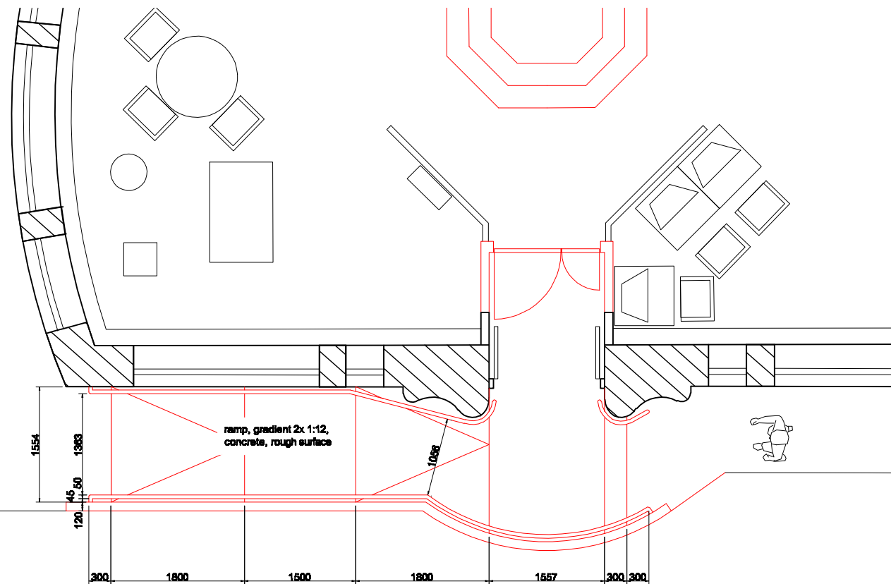
ground plan 1:50
